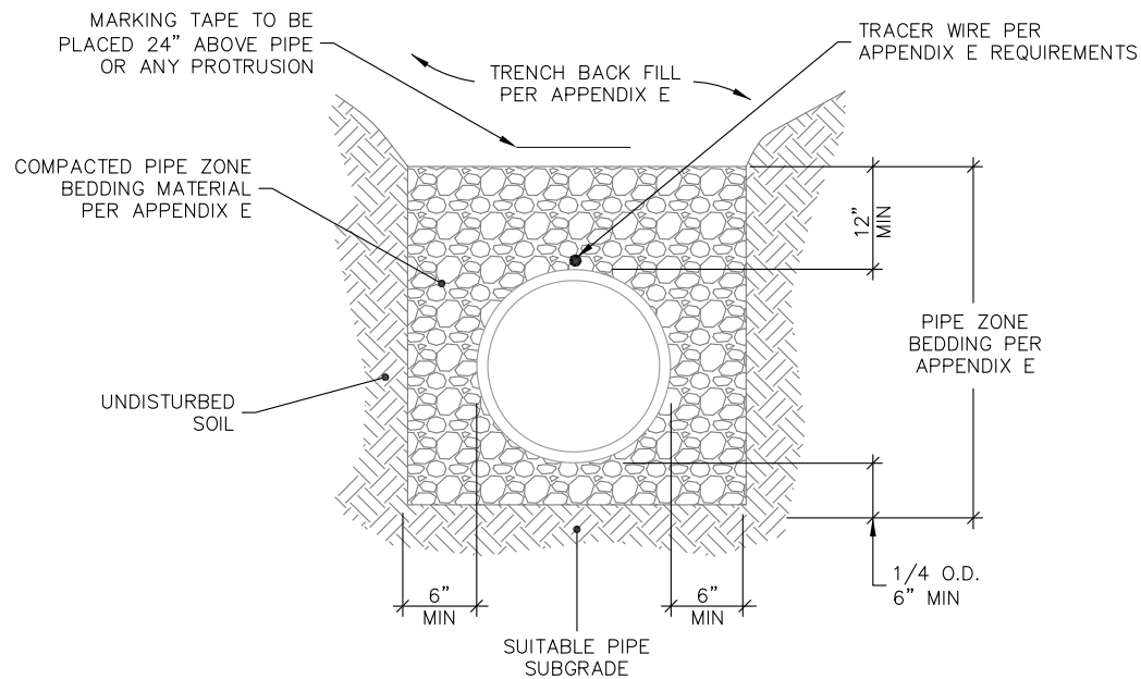
PIPE BEDDING ZONE
